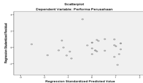
Figure 2 Heteroscedasticity Test
